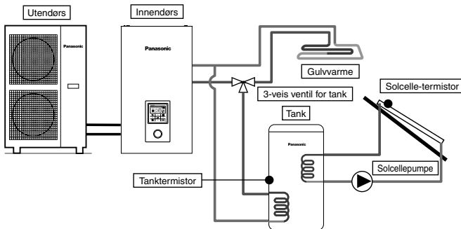
Tank + solcelletilkobling
